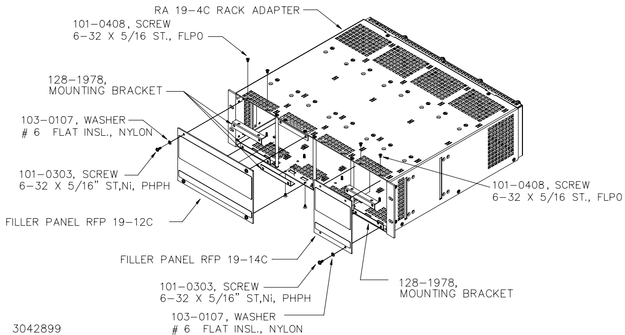
FIGURE 1. FILLER PANEL INSTALLATION
