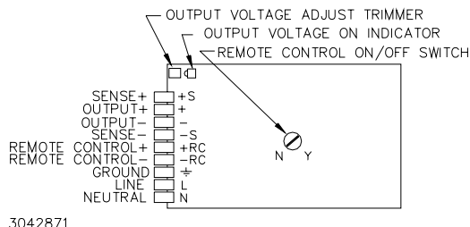
FIGURE 3. COMPONENT LOCATIONS
