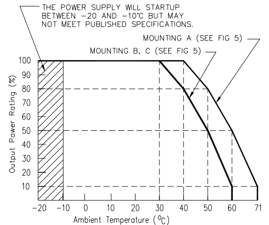
FIGURE 2. OUTPUT POWER VS. TEMPERATURE, KC MODELS (WITH COVER)
