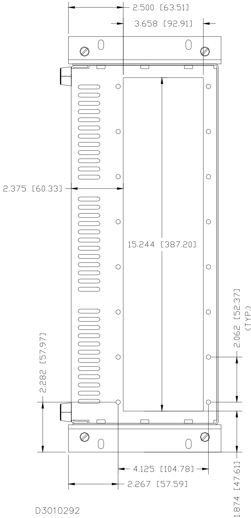
FIGURE 2. RA 79 RACK ADAPTER OUTLINE DRAWING (SHEET 3 OF 3, REAR VIEW)
