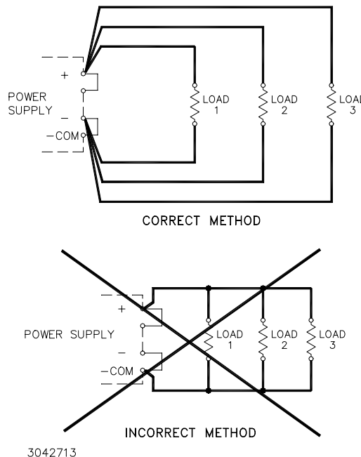
FIGURE 2. LOAD CONNECTIONS
