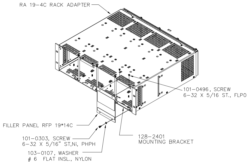
FIGURE 1. FILLER PANEL INSTALLATION
