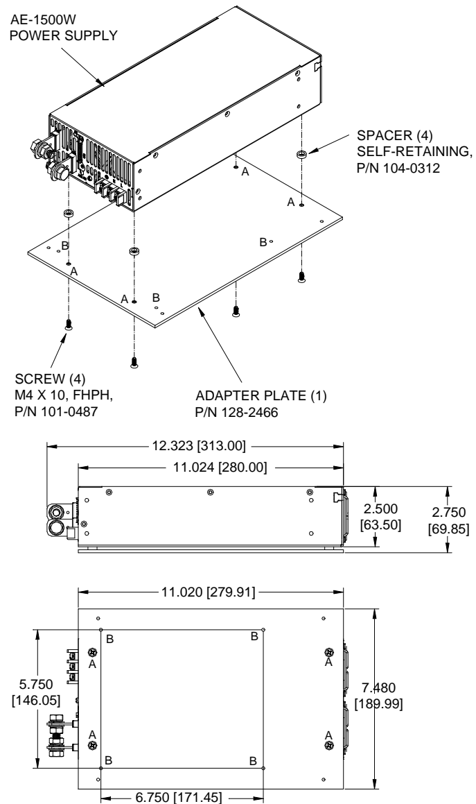
FIGURE 1. ADAPTER PLATE INSTALLATION
