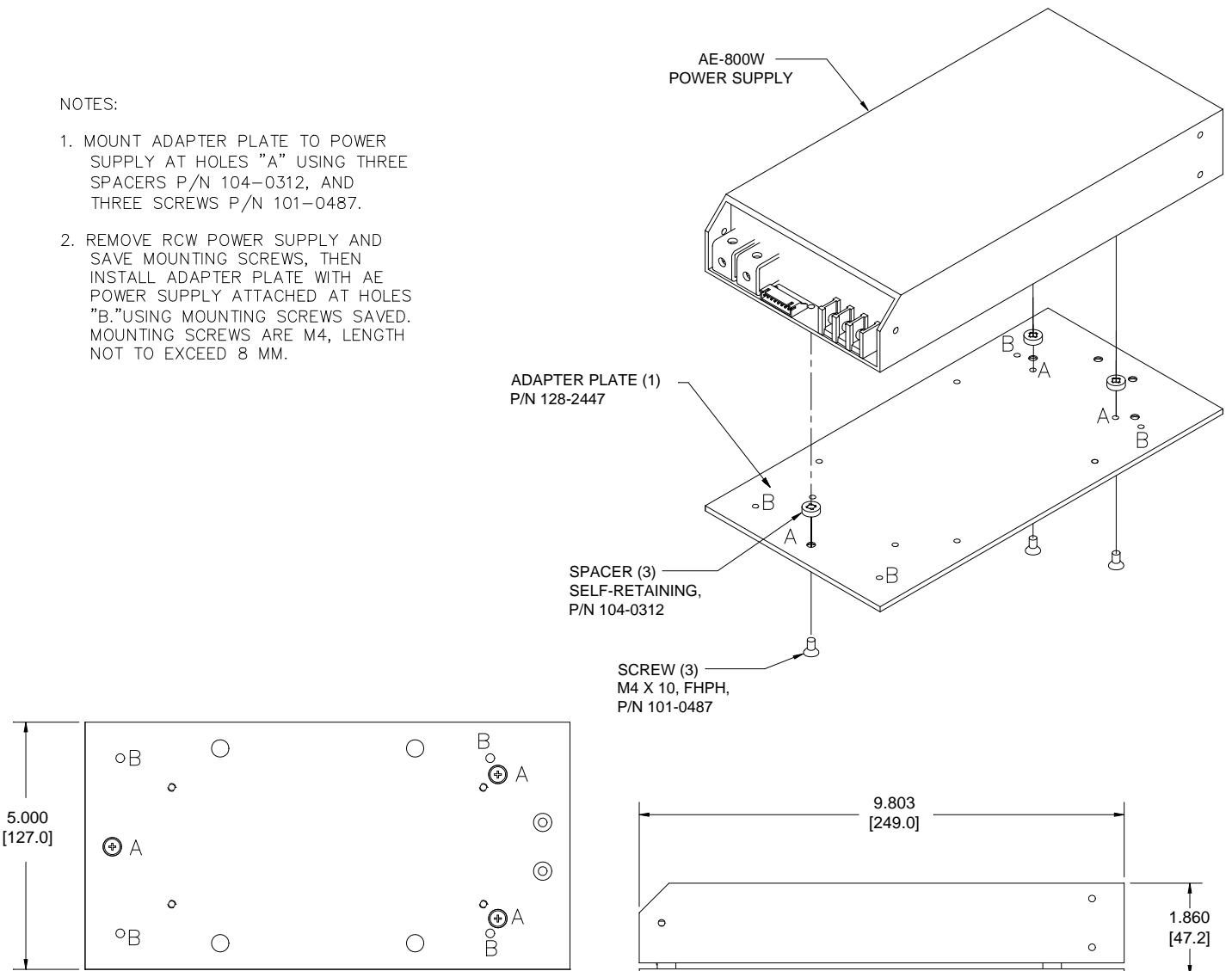
FIGURE 1. ADAPTER PLATE INSTALLATION
