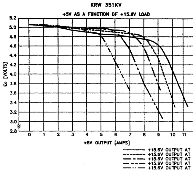
FIGURE 1 +5 V OUTPUT AS A FUNCTION OF +15.6V LOAD
